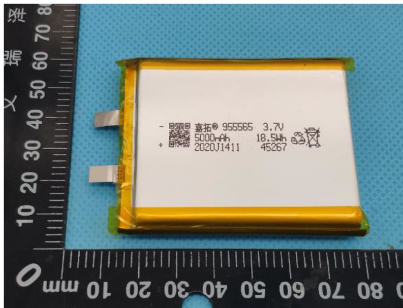
Figure 1 Front view of cell
